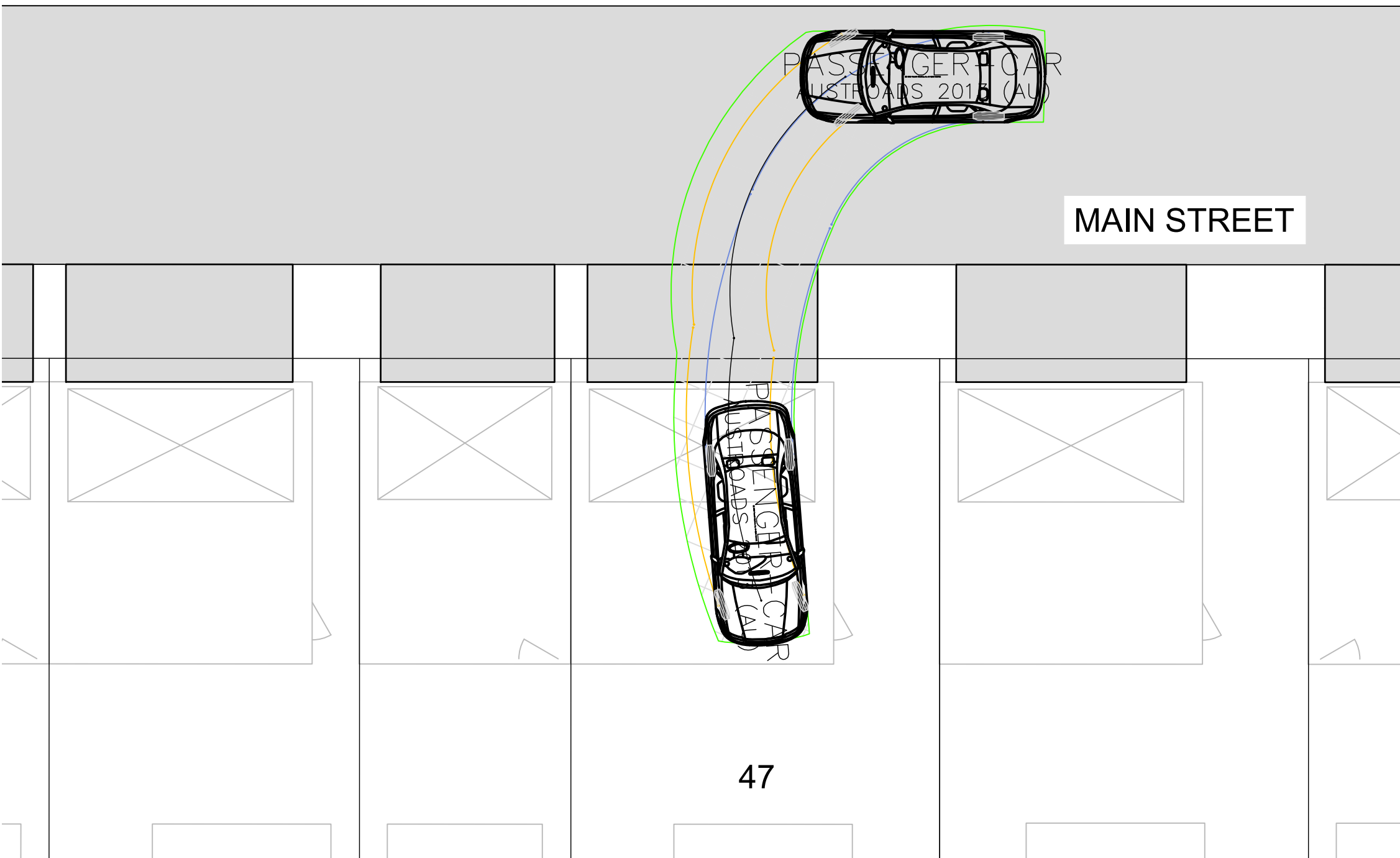
DRIVEWAY -DOUBLE GARAGE SCALE 1:100
