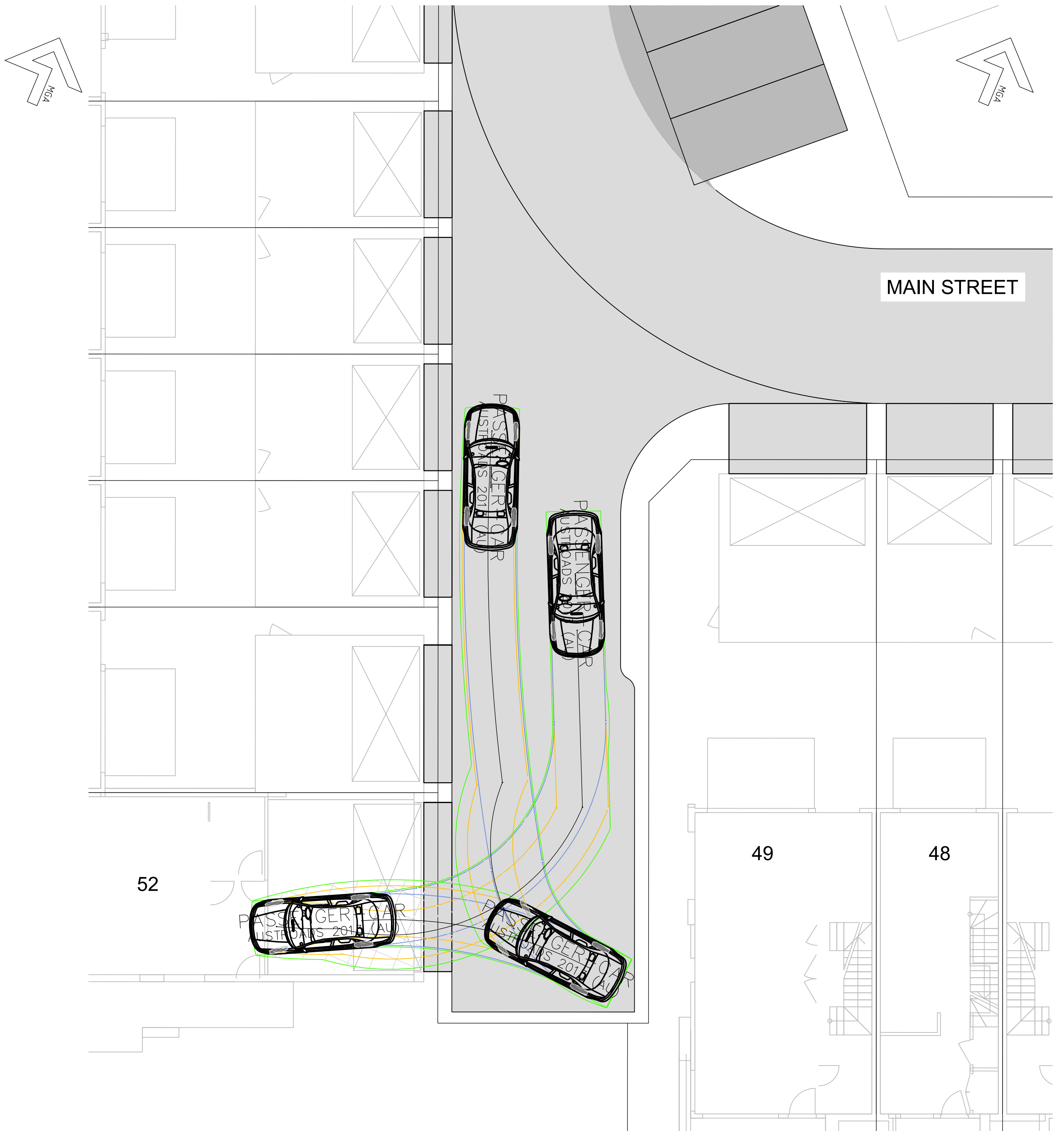
SOUTHERN DRIVEWAY - CAR TURNING PATH SCALE 1:100
